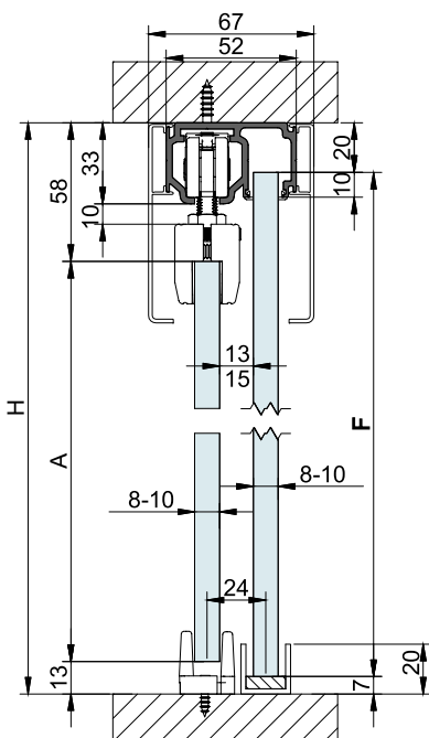
EXCELLENCE VIDRIO FIJO | FIXED GLASS | VERRE FIXE
