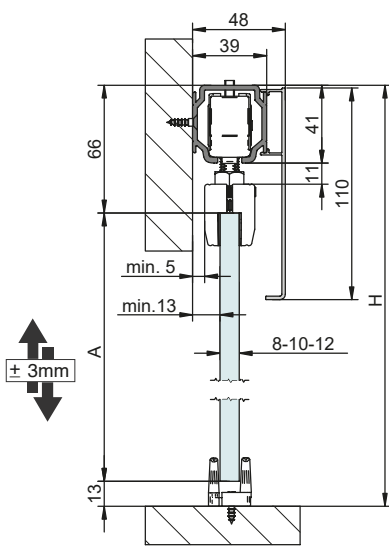
STANDARD XL A= H-79
