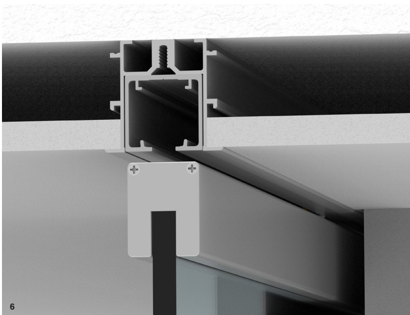
1, 2 y 3 Conjunto perfil Funda FT + Perfil Star, montaje a falso techo | Support FT + Star track set, false ceiling mounting | Ensemble Rail de couverture FT + Star, fixation a faux-plafond. 4, 5 y 6 Conjunto perfil Funda FT + Perfil Star, montaje entre paredes | Support FT + Star track set, mounting between walls | Ensemble Rail de couverture FT + Star, fixation entre les murs.
