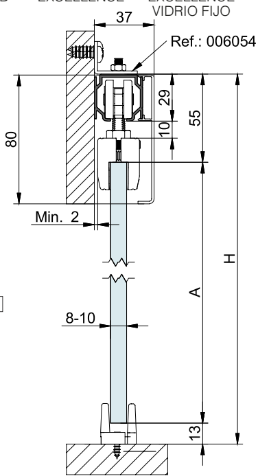
STANDARD A= H-68
