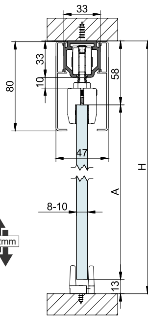
EXCELLENCE A= H-71
