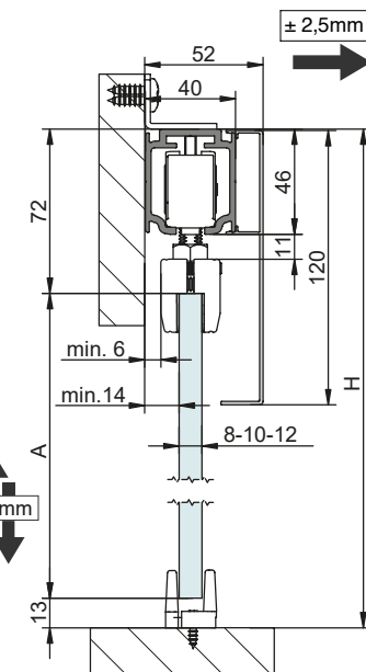
EXCELLENCE XL A= H-85
