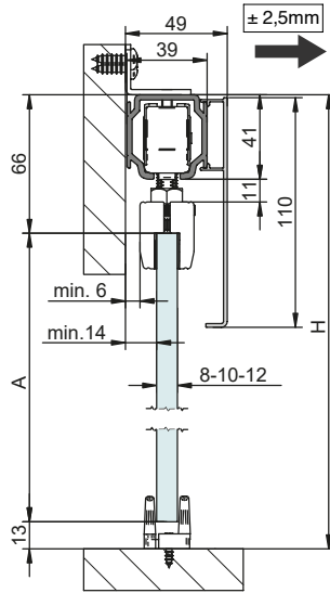
STANDARD XL A= H-79
