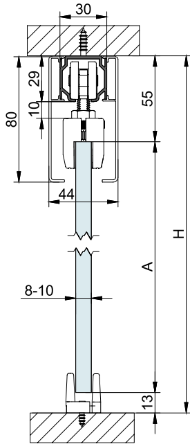
STANDARD A= H-68
