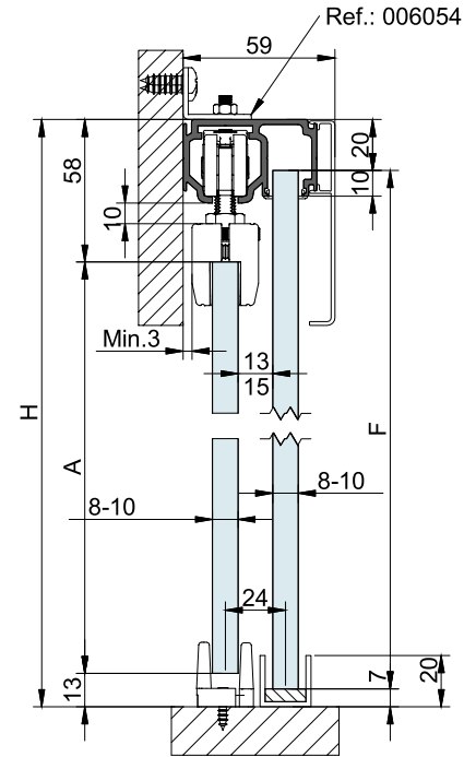
EXCELLENCE VIDRIO FIJO | FIXED GLASS | VERRE FIXE A= H-71 | F= H-29
