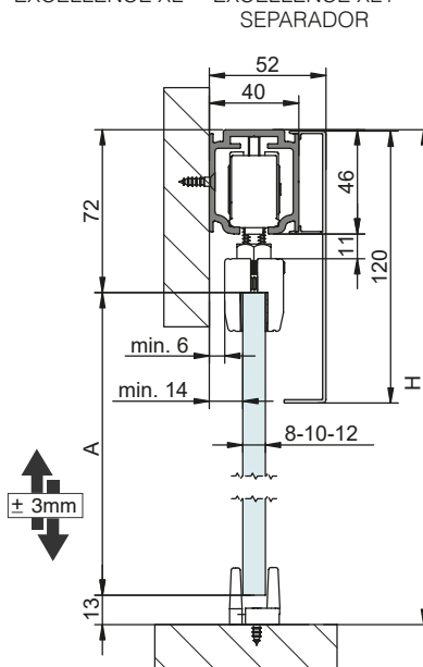
EXCELLENCE XL A= H-85
