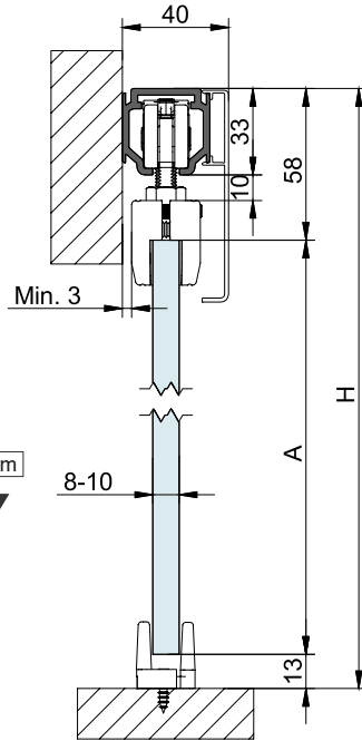
EXCELLENCE A= H-71
